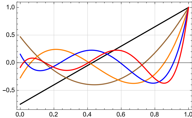
FIGURE 1. Normalized polynomials z \mapsto \hat{p}_n(z)/\hat{p}_n(1) on [0, 1] for n = 1(1)5
